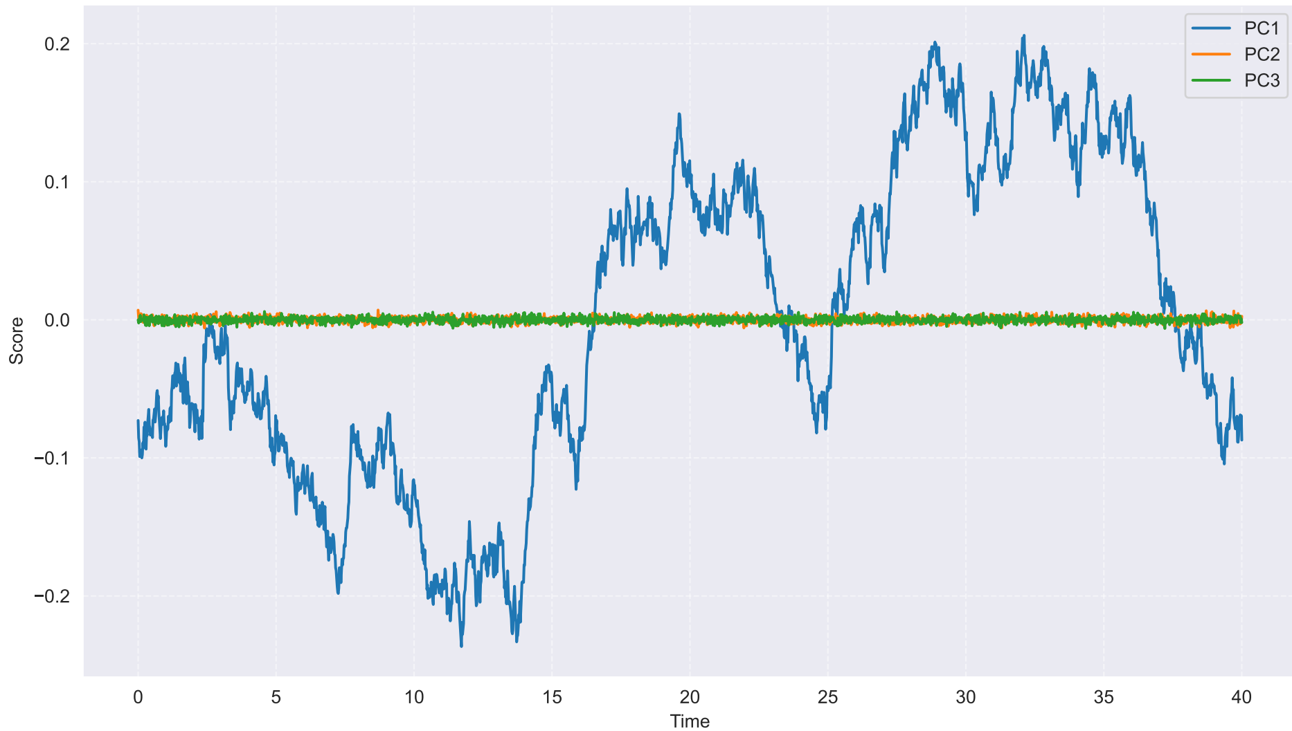
PCA Factor Time Series
